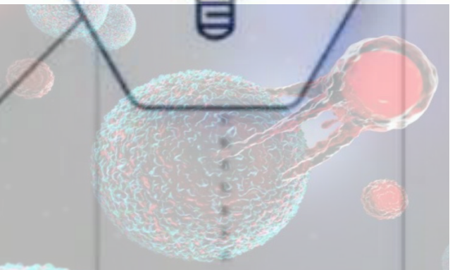
CAR-T
